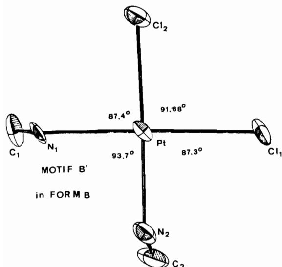
Fig. 2. View of the molecule B' implied in Form B.
