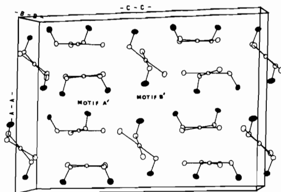
Fig. 3. Drawing of the molecular arrangement in crystal of the two different motifs showing favorable intermolecular interactions.
